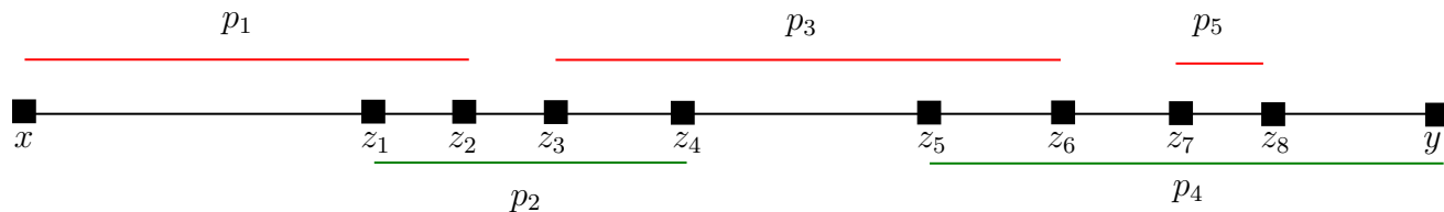
FIGURE 2. A schematic of the geodesic [x, y] traveling through several product regions.
